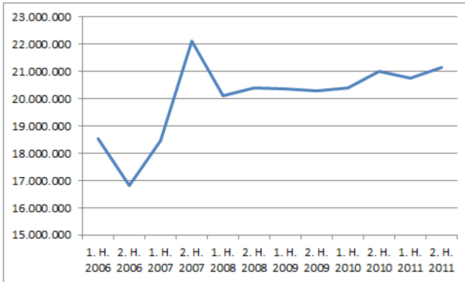
Figure 27. SMS sent
